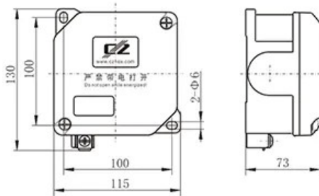
Modular type terminal box
