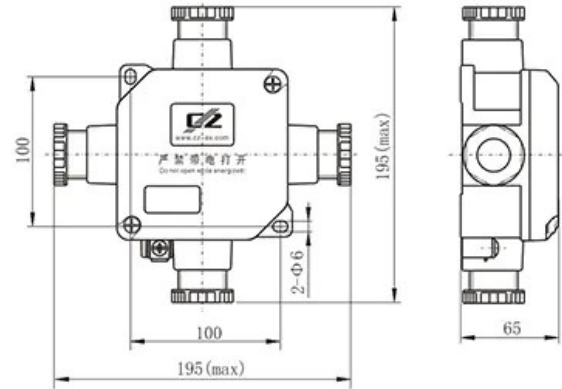
Fixed type terminal box
