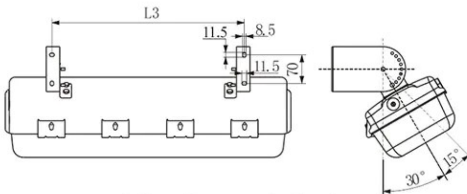
Adjustable mounting bracket
