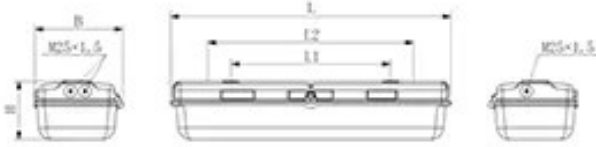
Full plastic explosion-proof (emergency) fluorescent light fittings
