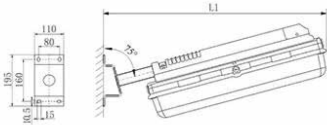
D8739 Wall mounting bracket of pole type
